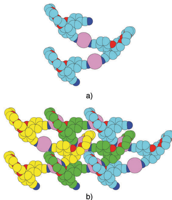
Fig. 9 A portion of the 2-D interwoven chiral network formed between 5 and \text{Ag}^+ . The entanglement between consecutive helical strands (a) of the same handedness is due to the interactions between the O atoms of the pentaethylene glycol units of 5 adopting a loop type arrangement within each strands and metal cations belonging to consecutive strands (b). For sake of clarity, carbon atoms belonging to different strands are differentiated by colour and H atoms and anions are not represented. For bond distances and angles see text.
