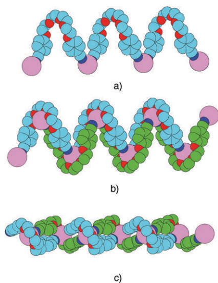
Fig. 8 A portion of the 1-D interdigitated network formed between 4 and \text{Ag}^+ . The interdigitation between the two helical strands (a) of the opposite handedness is due to the interactions between the O atoms of the tetraethylene glycol units of the tecton 4 adopting a loop type conformation within one strand and metal cations belonging to other strand (b and c). For sake of clarity, carbon atoms belonging to different strands are differentiated by colour and H atoms and anions are not represented. For bond distances and angles see text.
