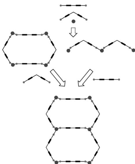
Fig. 5 Schematic representation of the two possible descriptions for the formation of the stair type architecture observed when the tecton 1 was combined with silver cation.
