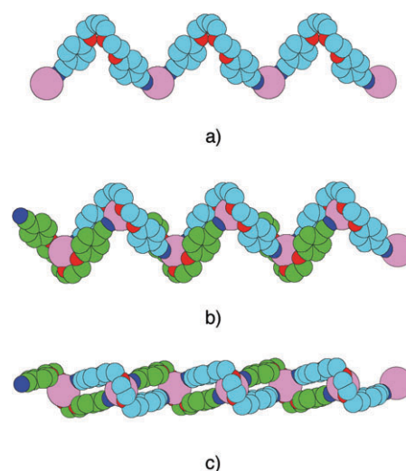
Fig. 6 A portion of the 1-D interdigitated network formed between 3 and \text{Ag}^+ . The interdigitation between the two helical strands (a) of the opposite handedness is due to the interactions between the oxygen atoms of the triethylene glycol units of the tecton 3 adopting a curved conformation within one strand and metal cations belonging to the other strand (b and c). For sake of clarity, carbon atoms belonging to different strands are differentiated by colour and H atoms and anions are not represented. For bond distances and angles see text.
