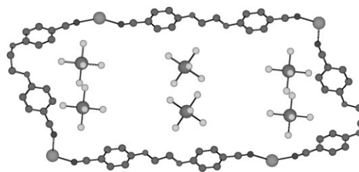
Fig. 3 A portion of the 1-D stair type coordination networks formed between 1 and \text{Ag}^+ cation showing the cyclic fragment and the positioning of the anions. For sake of clarity, H atoms are not represented. For bond distances and angles see text.
