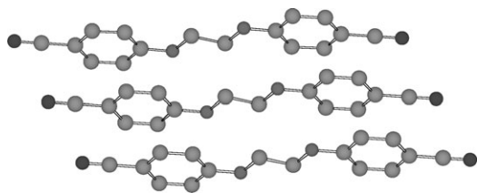
Fig. 1 The solid state structure of 1 showing the anti conformation adopted by the ethylene glycol moiety and the packing of consecutive units. For the sake of clarity, H atoms are not represented. For bond distances and angles see text.
