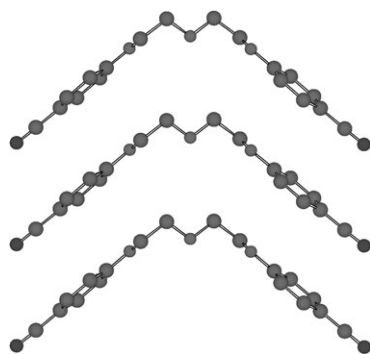
Fig. 2 A portion of the solid state structure of 2 showing the gauche conformation adopted by the ethylene glycol moieties and the packing of consecutive units. For sake of clarity, H atoms are not represented. For bond distances and angles see text.
