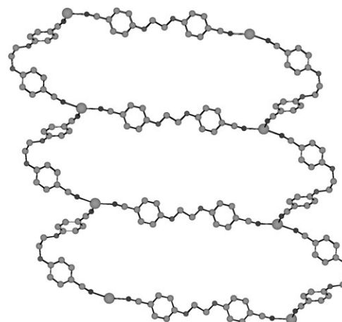
Fig. 4 A portion of the 1-D stair type coordination networks formed between 1 and \text{Ag}^+ cation showing the interconnection of the cyclic units by the tecton 1 . For sake of clarity, H atoms and anions are not represented. For bond distances and angles see text.
